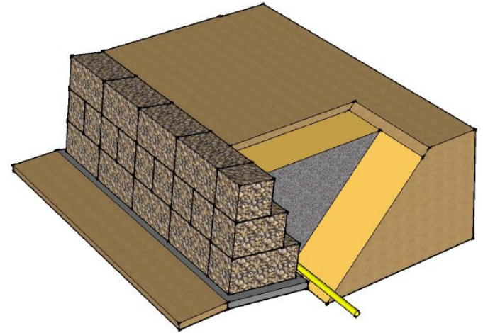
Gabion basket gravity wall
