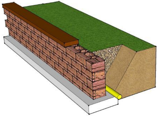
Keystone gravity wall
