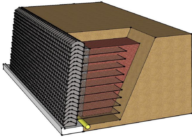
Chevloc reinforced soil wall
