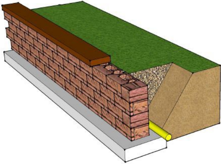
Keystone gravity design
