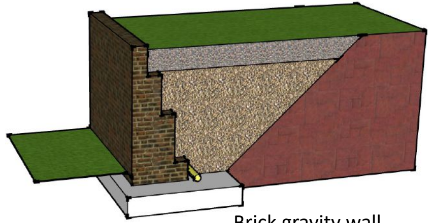
Brick gravity wall
