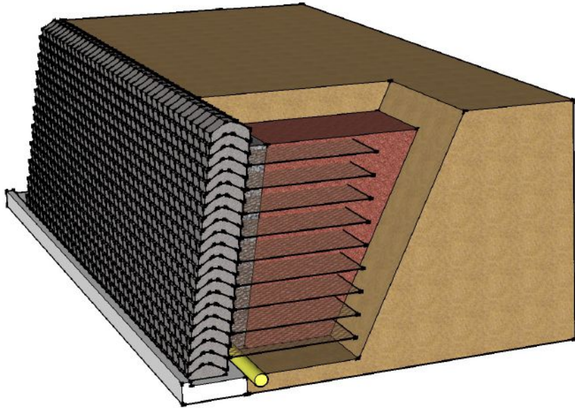
Chevloc reinforced soil design
